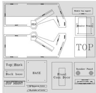
(a) Dynamo HS-1 schematics.
