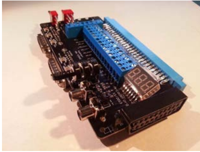
(a) Arcade Forge SuperGun MAK Strike. Image © arcadeforge.net.
